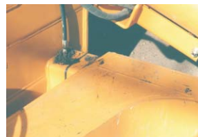
Ball Joint Connections with Hardened Socket Liners and Optional Central Lubrication
